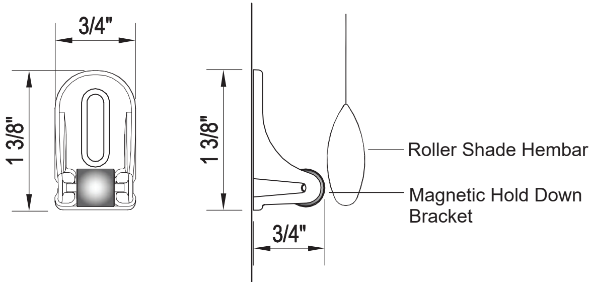
Installation Diagram
